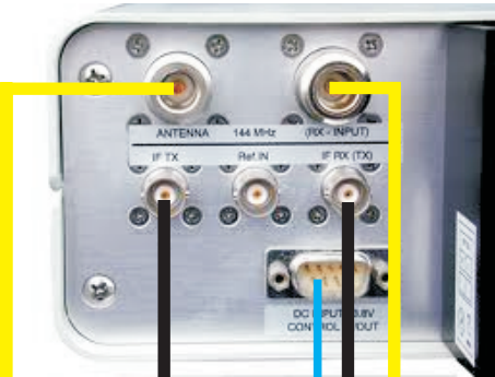
DB6NT 144/40
