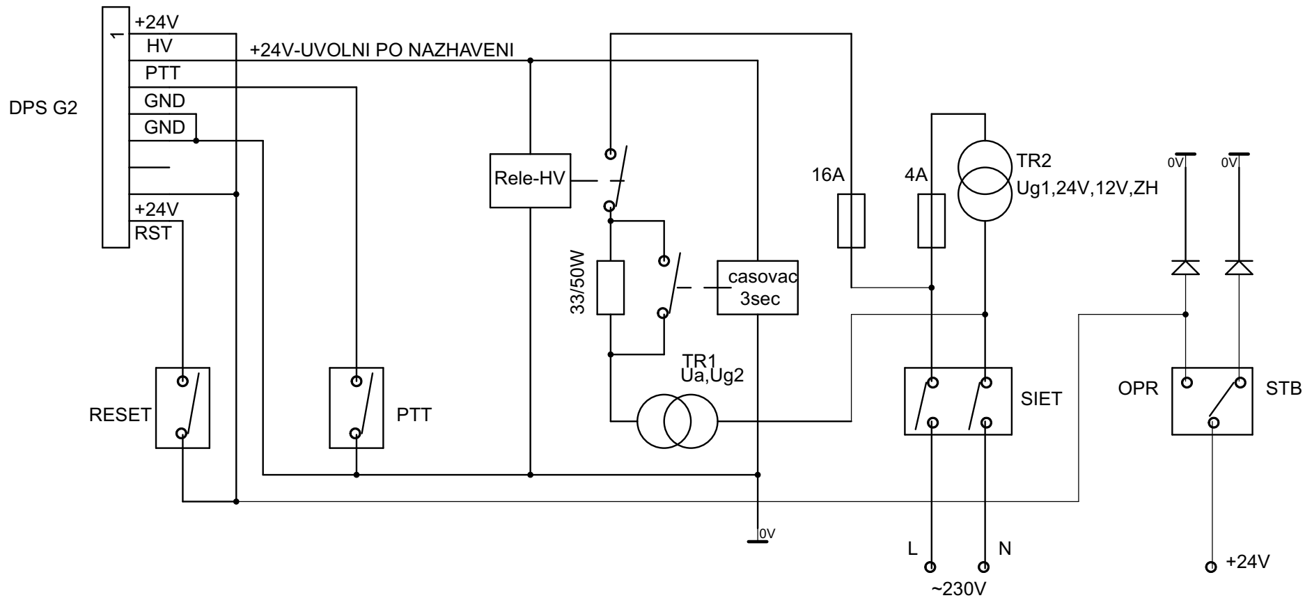
VBLOKOVE SCHEMA OVLADANIA CAST 1
